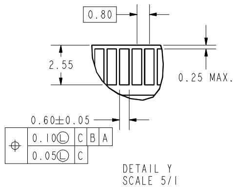
Figure 5: SO-DIMM Mechanical Drawing (3 of 5)
