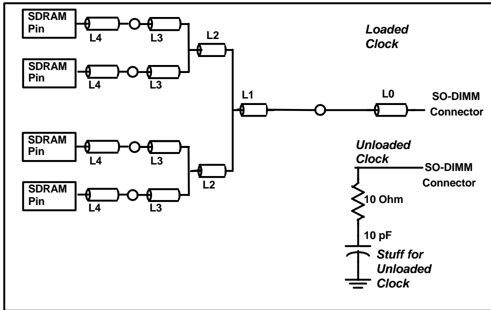
Figure 11: Signal routing topologies for Clocks
