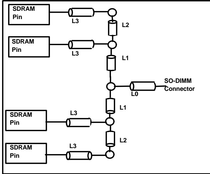
Figure 16: Signal routing topologies for Clock Enable
