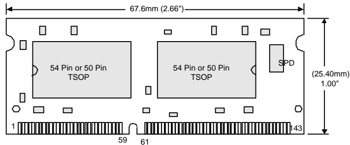
Figure 2: SO-DIMM with two 54-pin or 50-pin SDRAM per side
